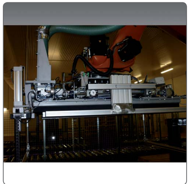
Special bolster gripper
